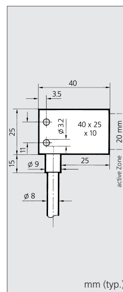
Winkel-Taster Angular scanner
