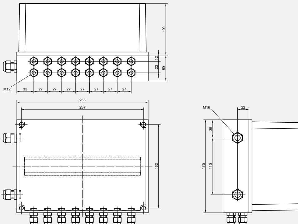
Protective enclosure PanBox 1x8 for one 8-channel amplifier
