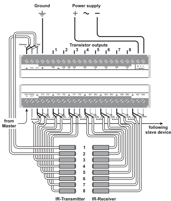
picture 2: Wiring diagram
