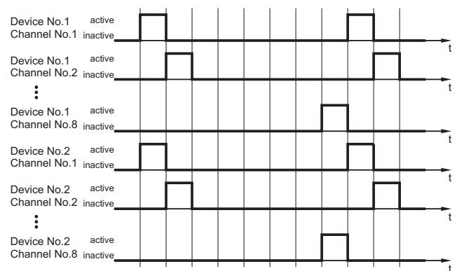
picture 4: Master-Slave operation
