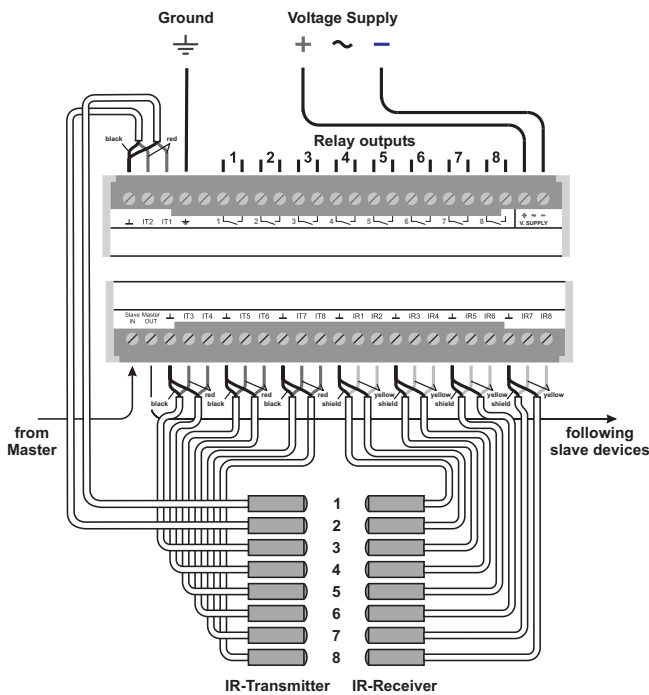
picture 2: Wiring diagram
